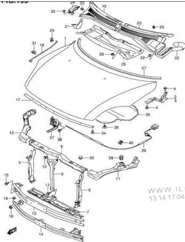
RS413 E22_195 FRONT HOOD PANEL
