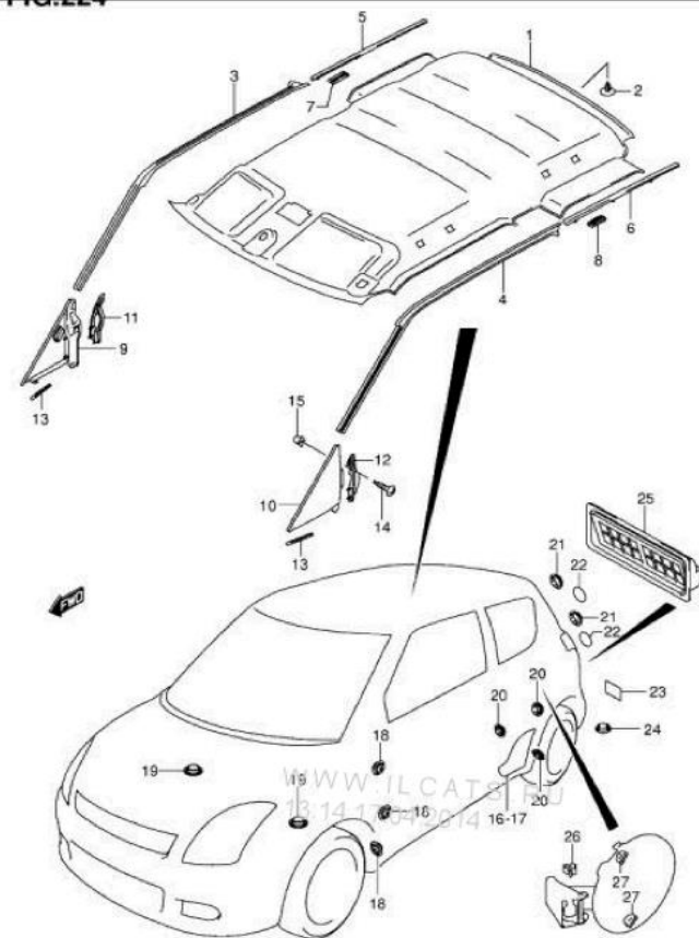
RS413 E22_224 ROOF LINING/ROOF MOLDING (3DR)
